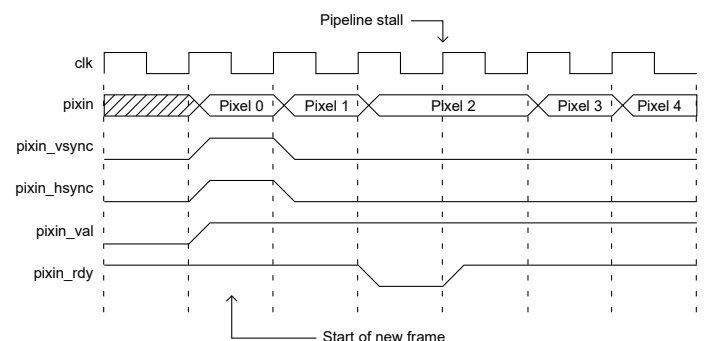
Figure 4: First line of a new input frame - also showing pipeline stall
