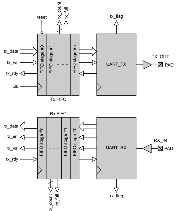
Figure 1: Simplified UART serial interface controller architecture
