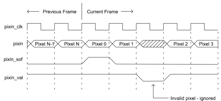
Figure 4: Input video interface timing
