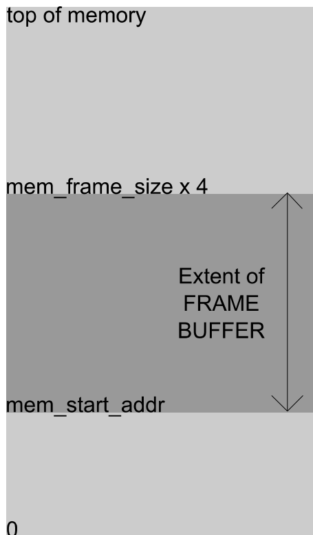
Figure 2: System memory map
