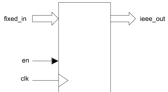
Figure 1: Fixed-point to 32-bit floating-point converter
