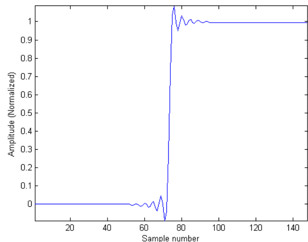
Figure 4: Step response of the 45-tap low-pass FIR filter
