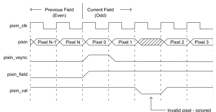
Figure 4: Input video interface timing
