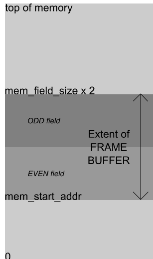
Figure 2: Frame buffer memory map
