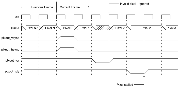
Figure 5: Output video interface timing - start of new output frame
