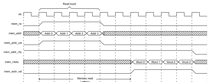
Figure 8: Memory read burst timing (burst size of 4)
