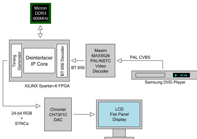
Figure 10: Block diagram of the development test setup
