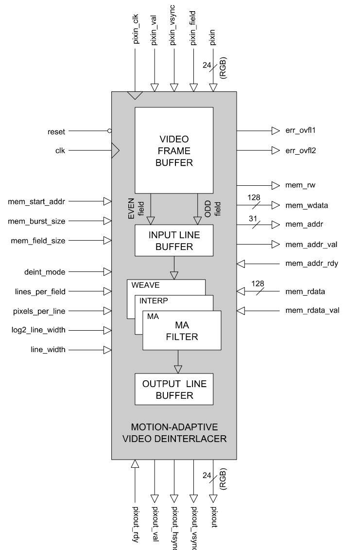
Figure 1: Motion-adaptive Video Deinterlacer Architecture
