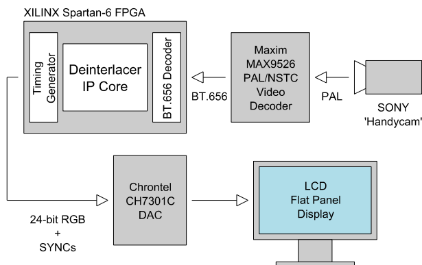
Figure 8: Development system hardware setup
