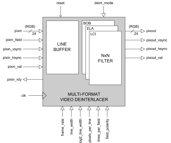
Figure 1: Video Deinterlacer Architecture
