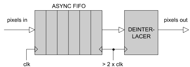
Figure 2: Deinterlacer clocking arrangement for maximum efficiency
